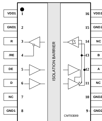
Figure 1-1. CMT83089 Pin List
