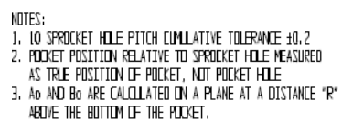
Figure 17. CMT83089 WB SOIC-16 Tape and Reel Information
