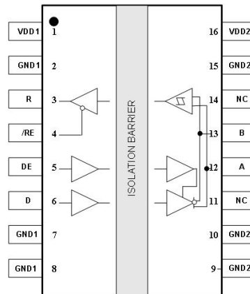
Figure 1-1. CMT83089C Pin List
