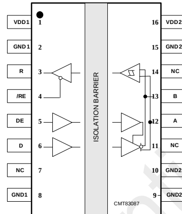
Figure 5-2. CMT83087 Pin List
