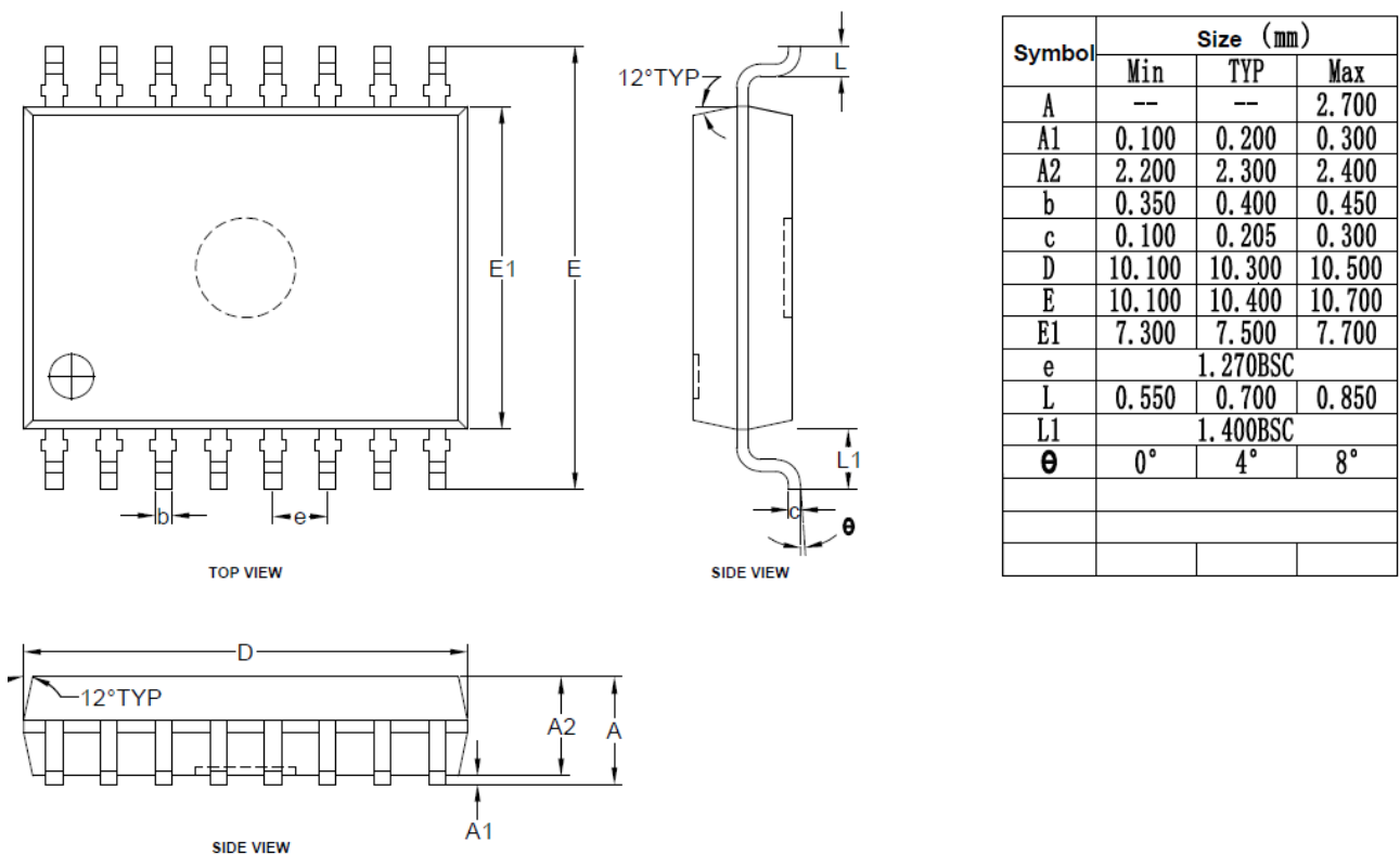
Figure 11-1. Wide Body SOIC-16 Packaging
