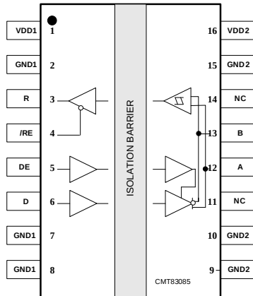
Figure 5-1. CMT83085 Pin List
