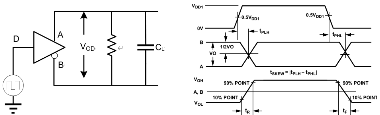
Figure 7-2. Driver Timing Test Circuit and Waveform
