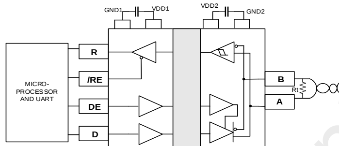
Figure 6-1. Typical Application Circuit
