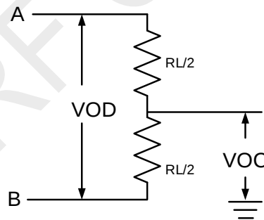
Figure 7-1. Driver DC Test Load
