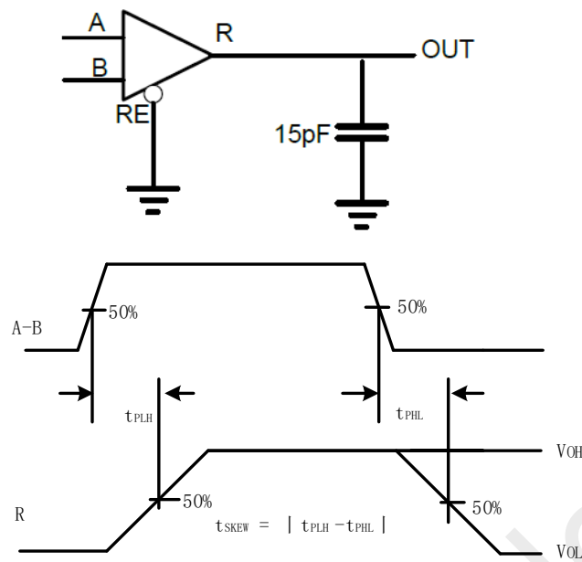
Figure 7- 4. Receiver Propagation Delay Test Circuit and Waveform
