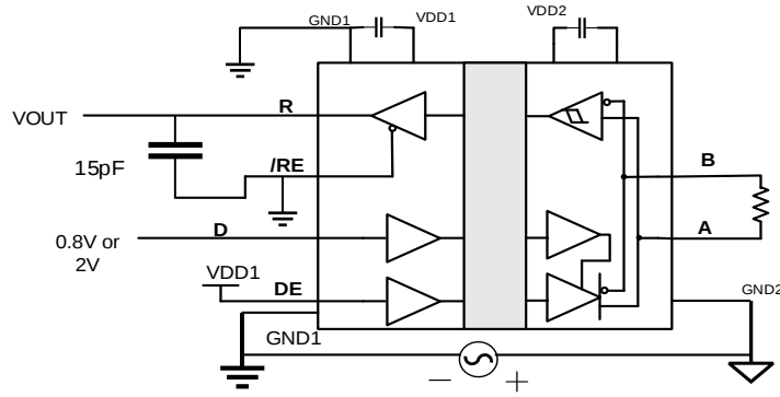
Figure 7- 6. Common-Mode Transient Immunity Test Circuit
