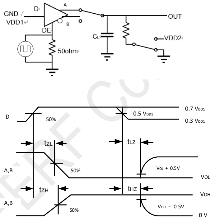
Figure 7-3. Driver Enable Disable Timing Test Circuit and Waveform
