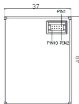
Figure 2 Connector Definition
