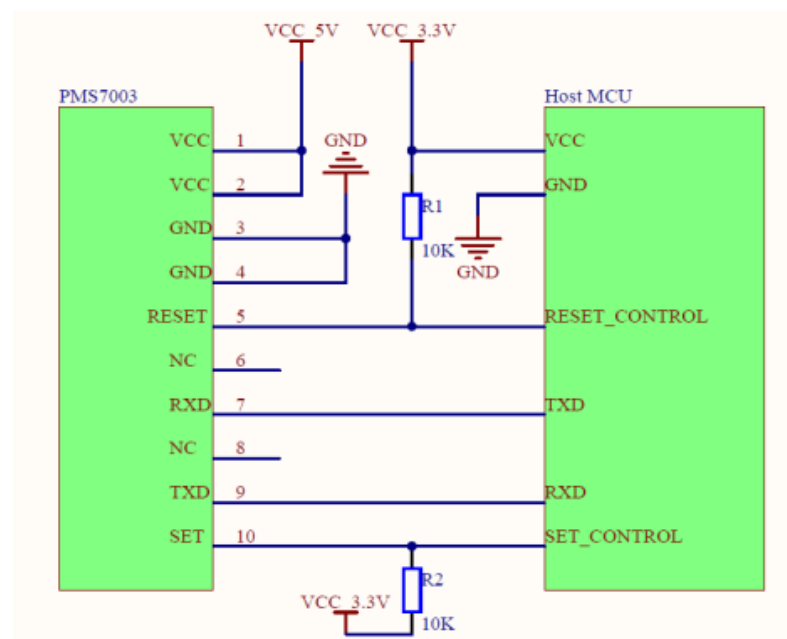
Figure 3 Typical Circuit
