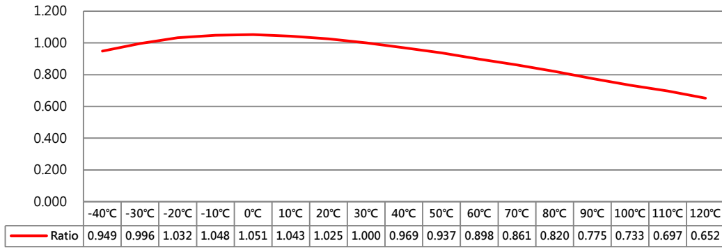
WCS7800 Sensitivity standardization of 30°C (3.3V) V.S Temperature
