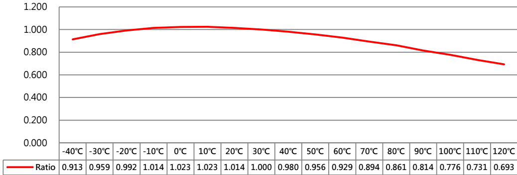
WCS7800 Sensitivity standardization of 30°C (5V) V.S Temperature
