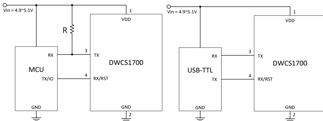
App. 1 Connect to MCU
